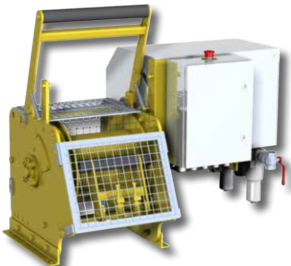
MR 30 FLG Weight: ~300 kg
